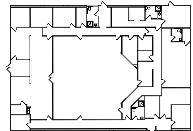
107'x75' Courtroom Building
