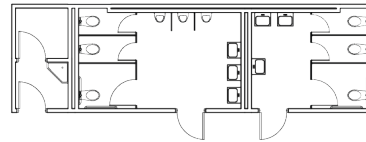
12'x40' Restroom Trailer
